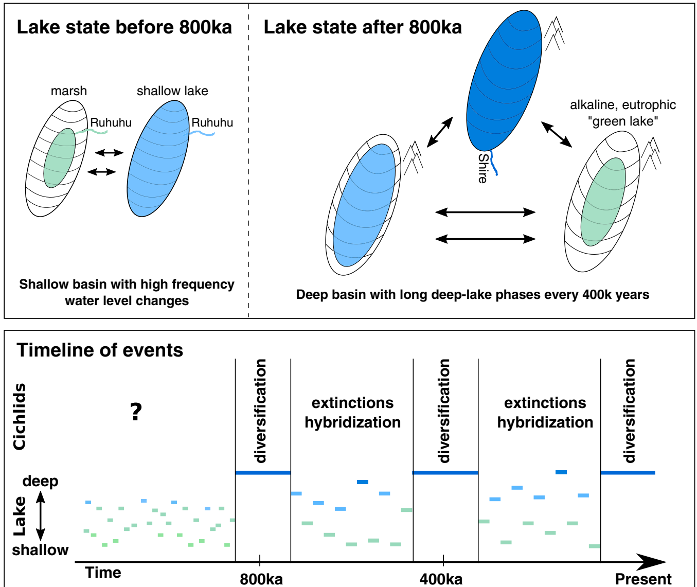
Fig. 1. The environmental history of Lake Malawi over the past 1.2 Ma and its interrelation with its cichlid adaptive radiation. According to Ivory et al. (1), the lake was characterized by frequent oscillations between marsh and shallow-lake conditions before 800 ka and had a constant outflow (the Ruhuhu River). After 800 ka, this outlet closed resulting in a much deeper and often closed basin (with an outflow via the Shire River only during highstands). Consistent with a recent molecular clock calibration (12), the cichlid radiation is likely to have kicked-off during the first phase of deep-lake conditions ~800 ka. This event might be equivalent to the first stage of adaptive radiation (14–16), the specializations to macrohabitats. Focusing on the rock-dwelling mbuna lineage, Ivory et al. (1) propose that two further deep-lake phases (~400 ka; since ~75 ka) might be responsible for trophic specializations (stage II) and diversification with respect to coloration (stage III). A more general hypothesis, which should be evaluated in the future, is that cichlid evolution was shaped by periods characterized by diversification and large population sizes during deep-lake phases, interspersed by periods characterized by unstable conditions, extinctions and interspecific gene-flow during lowstands.
